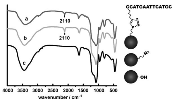
Figure 2. FTIR spectra of a) MCM-41, b) MSPs- \text{N}_3 , and c) MSPs-DNA.
